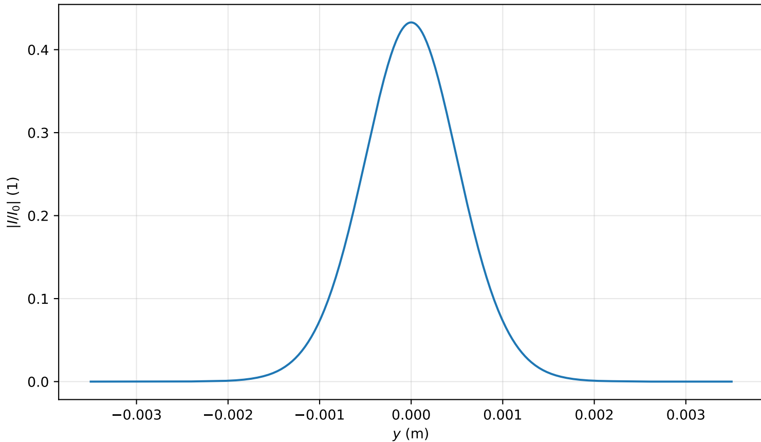
Intensity profile I(x=0, y, z=2.946)/I_0 , P_{in}=0.3P_{cr} , artificial time
